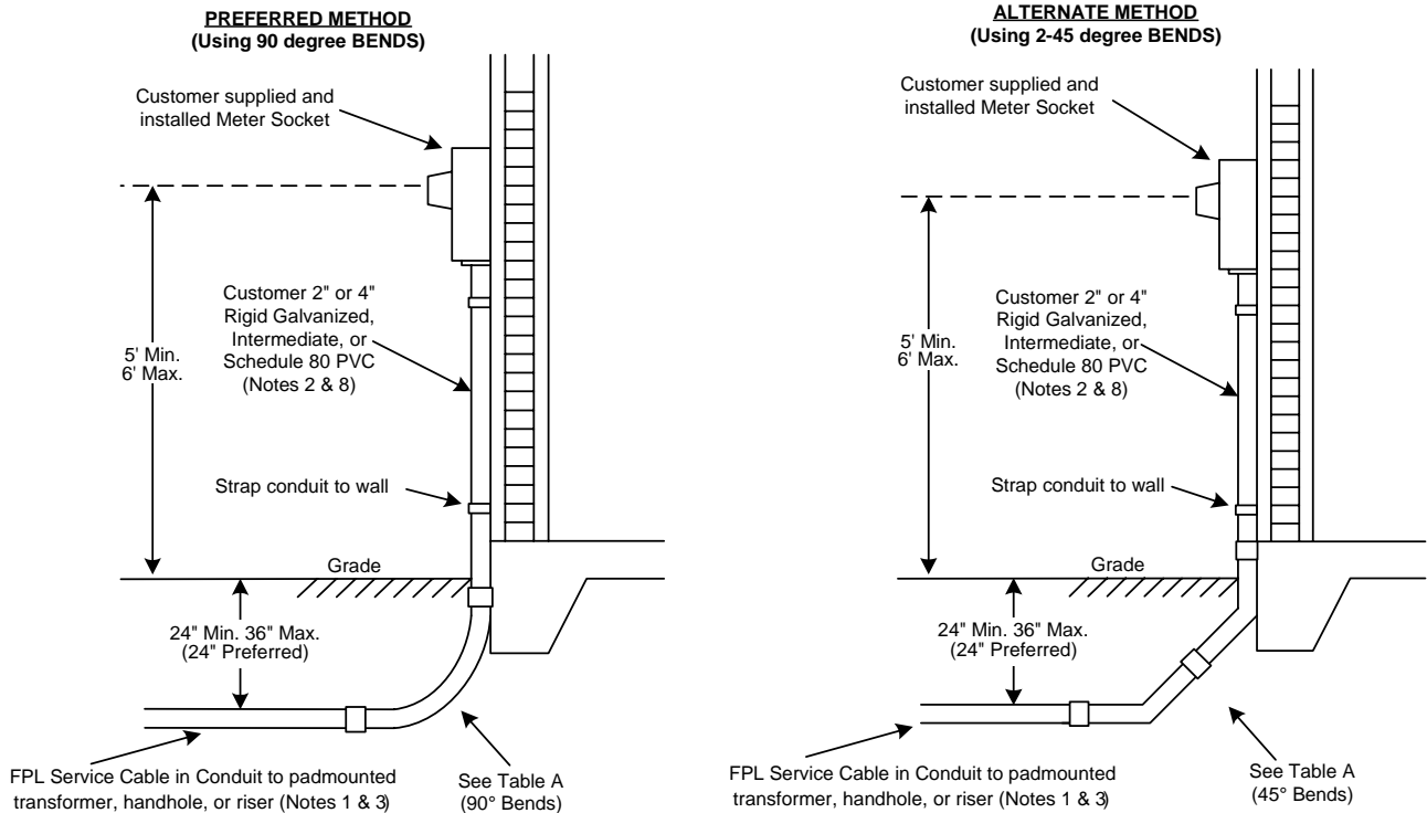
FIGURE IV-11b FPL Buried Service Lateral – Meter Socket & Down Pipe Requirements (references to notes shown in Figure IV-11a )
