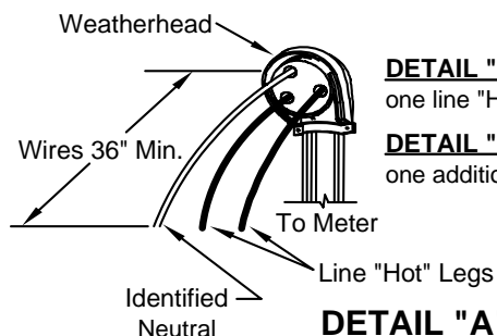
3-WIRE, 120/208Y 1ph (2 STATOR NETWORK) METER SYMBOL "E"
