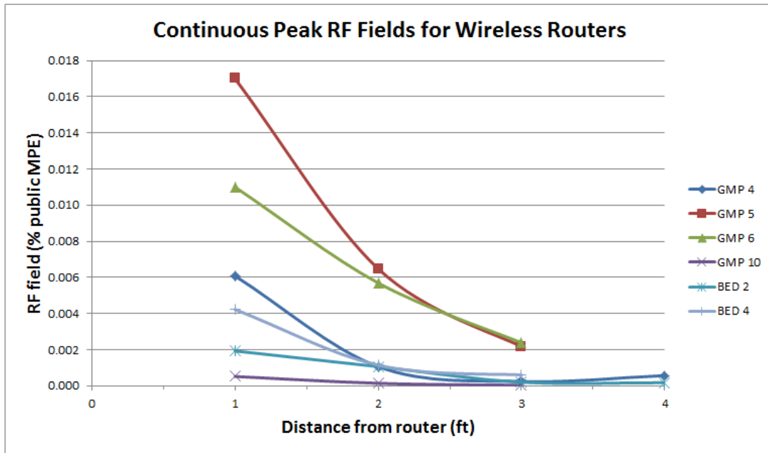
Figure 61. Spatial variation of peak RF fields continuously emitted by six wireless routers measured during this project.
